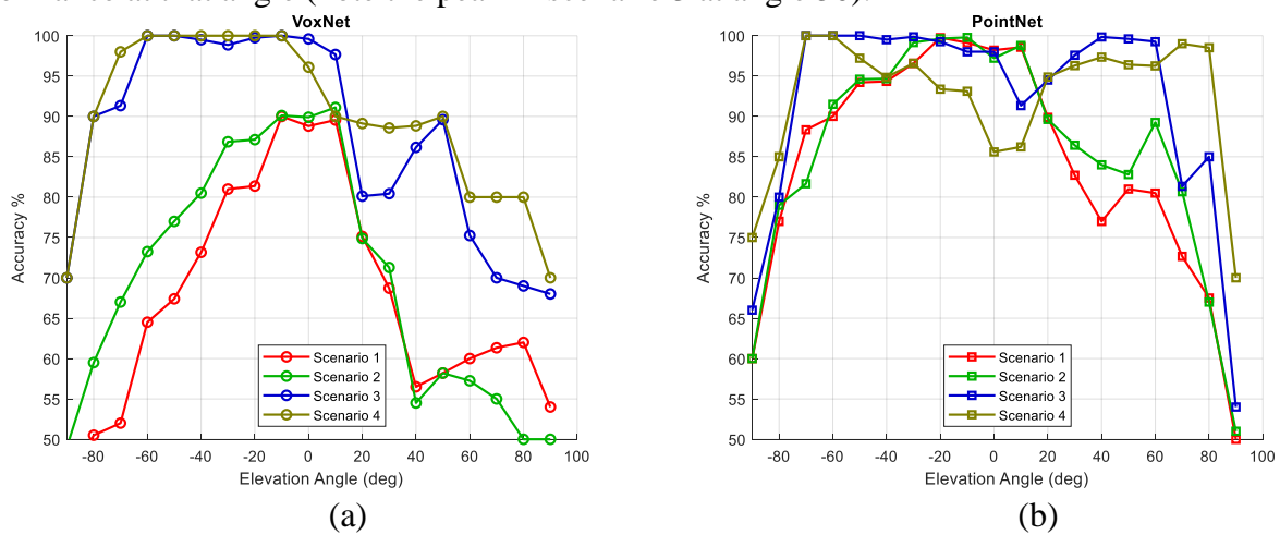
Figure 1 – Performance of deep learning classification using our created dataset for different training scenarios: (a) VoxNet classifier, (b) PointNet classifier
